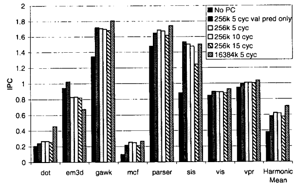
Figure 4. Performance impact when the main thread is permitted to access a pointer cache of varying sizes. All configurations also use the stride prefetcher. No PC refers to the baseline with only stride prefetching. Val pred only shows results using the pointer cache for only value prediction. All of the rest of the PC results use the pointer cache for both value prediction and prefetching.
