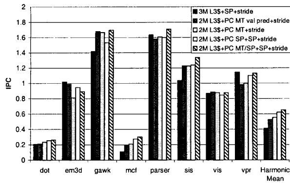
Figure 7. Performance results comparing a processor with a 2M 8-way L3 cache and 256k entry 4-way, 20 cycle pointer cache against a baseline stride prefetching architecture with a 3M, 12-way L3 cache. The pointer cache is used for value prediction and prefetching for all main thread (MT) results, except the second bar, where the pointer cache is only used by the main thread for value prediction. All configurations access their L3 cache in 30 cycles.
