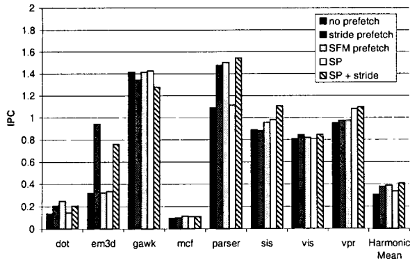
Figure 3. Performance improvement from previous prefetching schemes.
