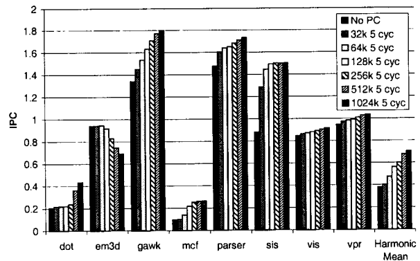
Figure 5. Performance impact varying the number of entries in the pointer cache. No PC refers to stride only prefetching. All the other configurations also make use of stride prefetching.
