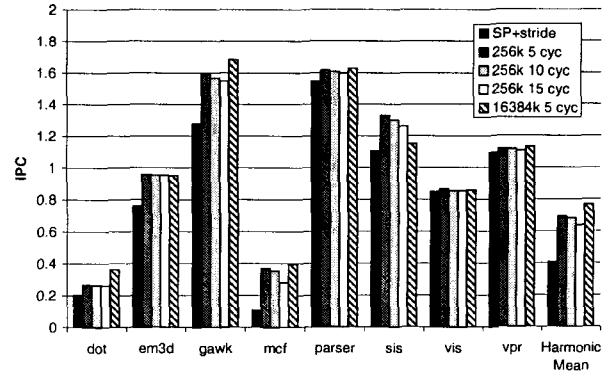
Figure 6. Performance impact from combining SP and stride prefetching when only using the pointer cache for speculative precomputation threads. The main thread does not use the pointer cache.
